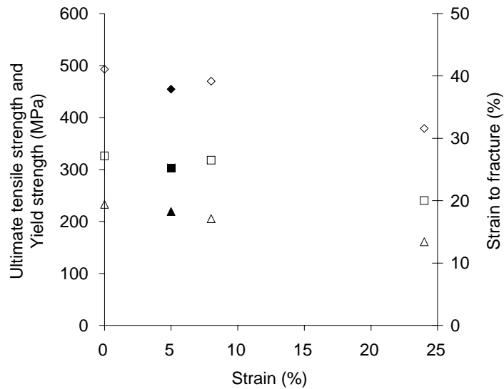
Figure 3: Mechanical properties of AA2024 in the T42 temper as a function of strain. Tensile strength ( \diamond, \blacklozenge ), yield strength ( \blacksquare, \square ), strain to fracture ( \blacktriangle, \triangle ). Material of batch A (solid) and batch B (open).
