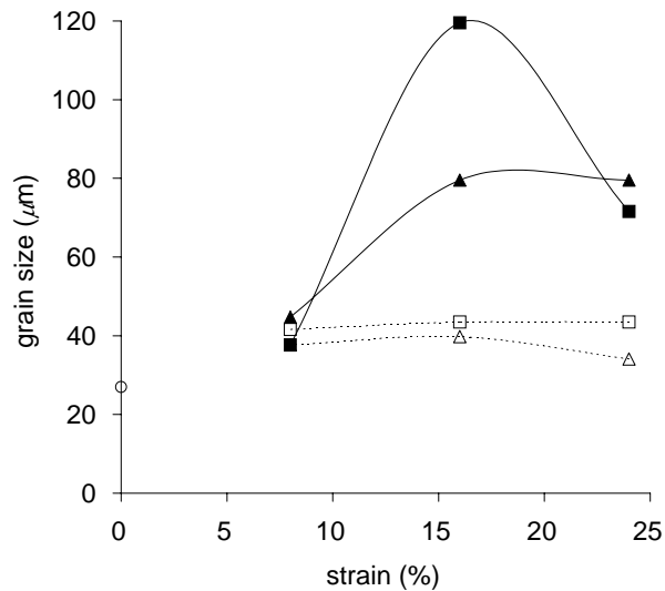
Figure 4: Grain size before the solution heat treatment (open) and in the T42 temper (solid) as a function of strain. Rolling direction ( \blacktriangle, \triangle ) and transverse direction ( \blacksquare, \square ).
