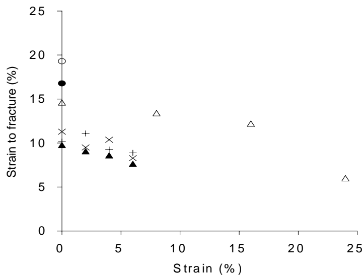
Figure 2: Strain to fracture of AA2024 T3 material (●,○) and after intermediate annealing as a function of strain (▲,△). Material of batch A (solid) and batch B (open). Transverse direction (⊕) and 45° to the rolling direction (×).
