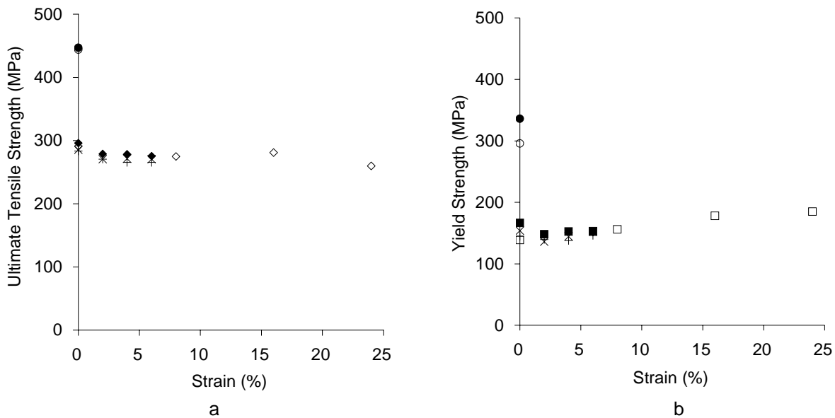
Figure 1: Tensile strength (a) and yield strength (b) of AA2024 T3 material (●,○) and after intermediate annealing as a function of strain. Tensile strength (◇,◆); Yield strength (■,□). Material of batch A (solid) and batch B (open). Transverse direction (⊕) and 45° to the rolling direction (×).
